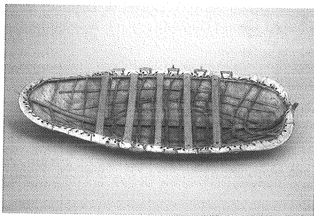
Figure 3. Unangax open skin boat ( nixalax ) model, collected by Ivan Kuprianov, chief manager of the Russian-American Company, ca. 1837. Photo: courtesy of the Natur und Mensch Museum, Oldenburg, Germany, item 303. Photographer: Gudrun Bucher.
