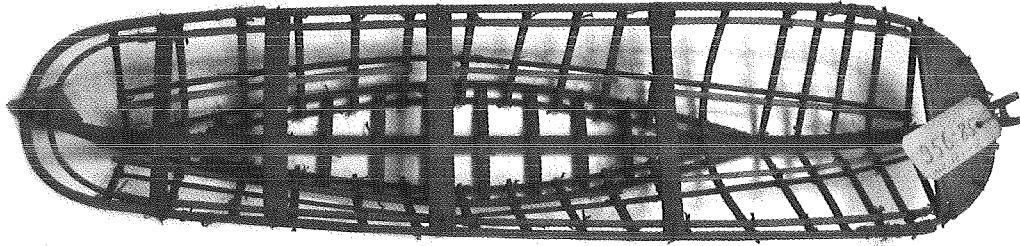
Figure 8. Koryak umiak frame model. Photo: courtesy of Peter the Great Museum of Anthropology and Ethnography (Kunstkamera), Russian Academy of Sciences, St. Petersburg, item MAE956-85.
