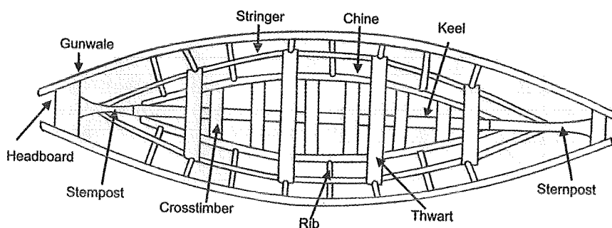
Figure 1. Parts of a classic umiak.
